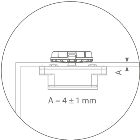
CEILING MOUNT
